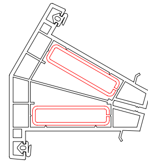
150° corner post reinforcement 116017 reinforcement 113028 aluminium reinf 115015 gasket 112003
