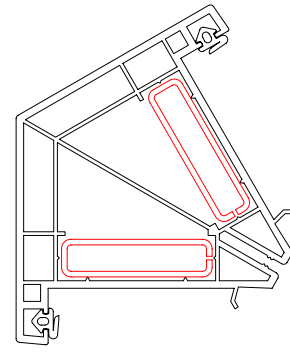
120° corner post reinforcement 116016 reinforcement 113028 aluminium reinf 115015 gasket 112003
