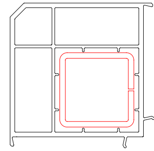
90deg Corner post reinforcement 116200 Steel reinforcement 113128 adjustment nut 141444 LOAD BEARING
