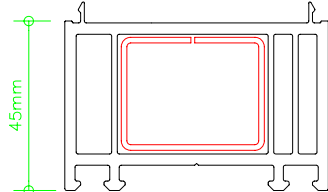
45mm frame extension 114202 Reinforcement 113271
