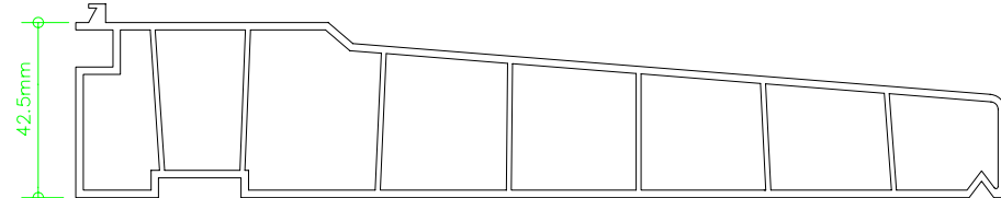
225mm Cill - 110.106 reinforcement - 113.048 & 345 end cap 109647
