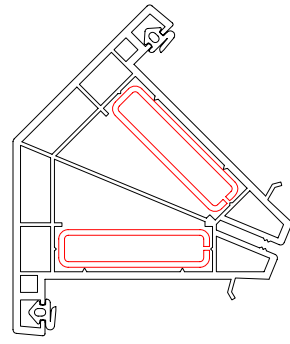
135° corner post reinforcement 116015 reinforcement 113028 aluminium reinf 115015 gasket 112003
